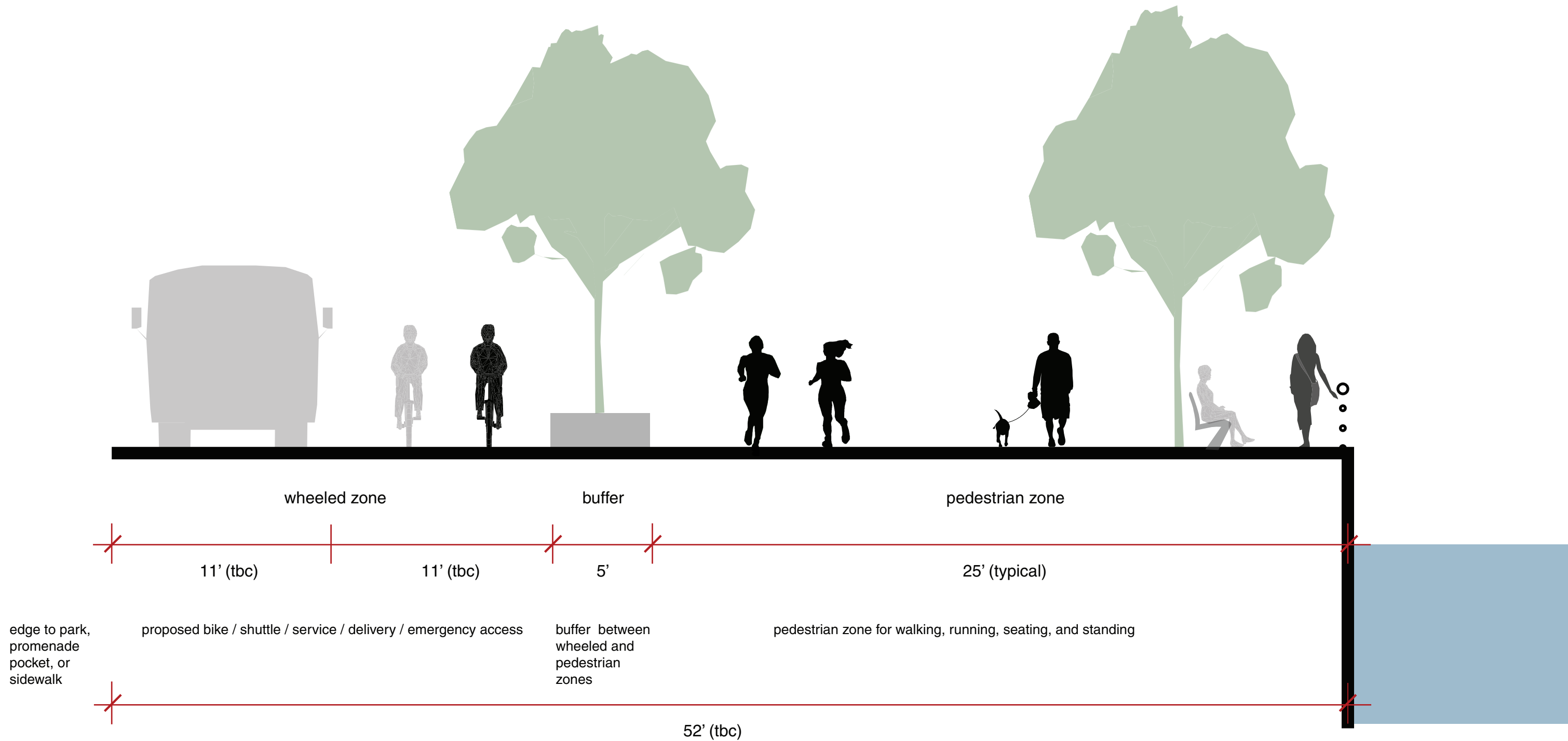
Figure 2 - The Great Promenade Typical Section
